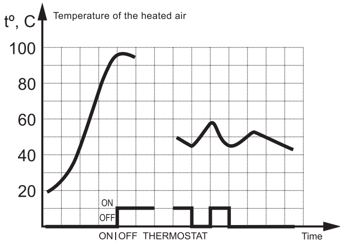
CHARACTERISTIC OF THE THERMOSTAT
